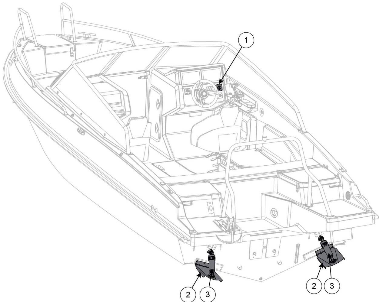
Figur 5.5 Cross 75 BR trimsystem
